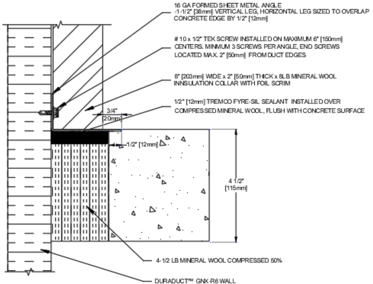
Typical Firestop Detail through floor assembly
