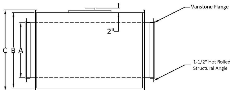
DuraDuct KEX Construction Detail
