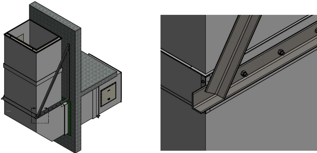
Typical Knee Bracket – Vertical Support
